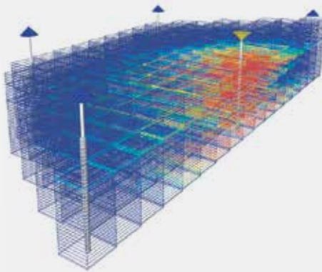
Model ASP and low salinity waterflood processes
